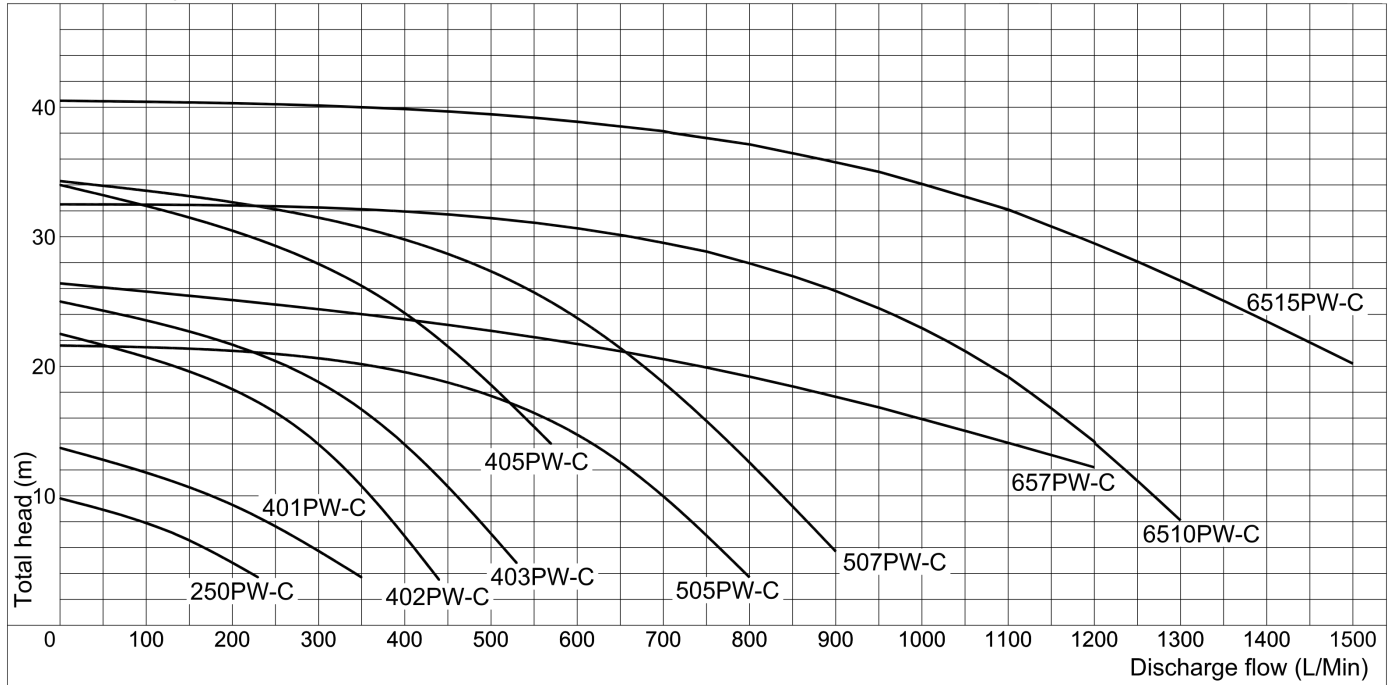
PW-C Family Curve 50Hz
